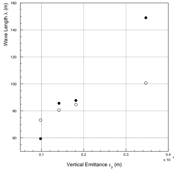
Fig. 13. Wavelength of the oscillation as a function of the vertical emittance.
