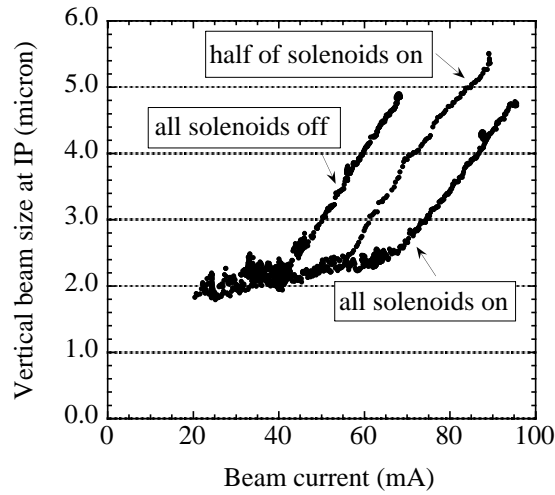
Fig. 6. Vertical beam size as a function of the beam current. In the measurement, two trains were injected on opposite sides of the ring. Each train contained 60 bunches. The bunch spacing was 4 rf buckets.
