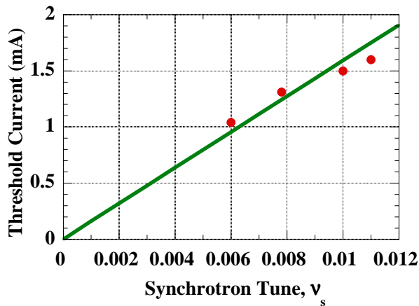
Fig. 15. Threshold bunch current of beam loss vs. synchrotron tune.
