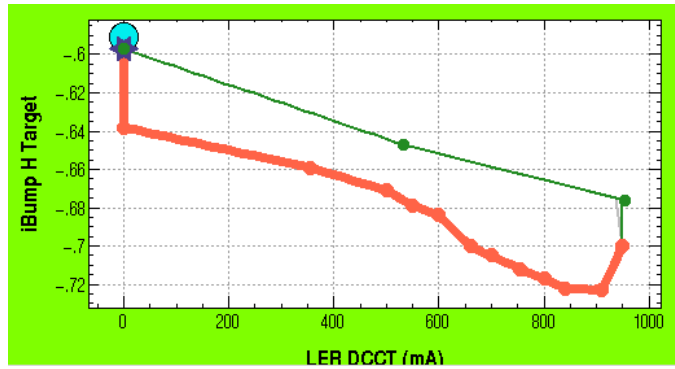
Fig. 22. Example of a diagram for the target value for \Delta x_{xcan}^* . The target is programmed to change as a function of the LER current during a fill.
