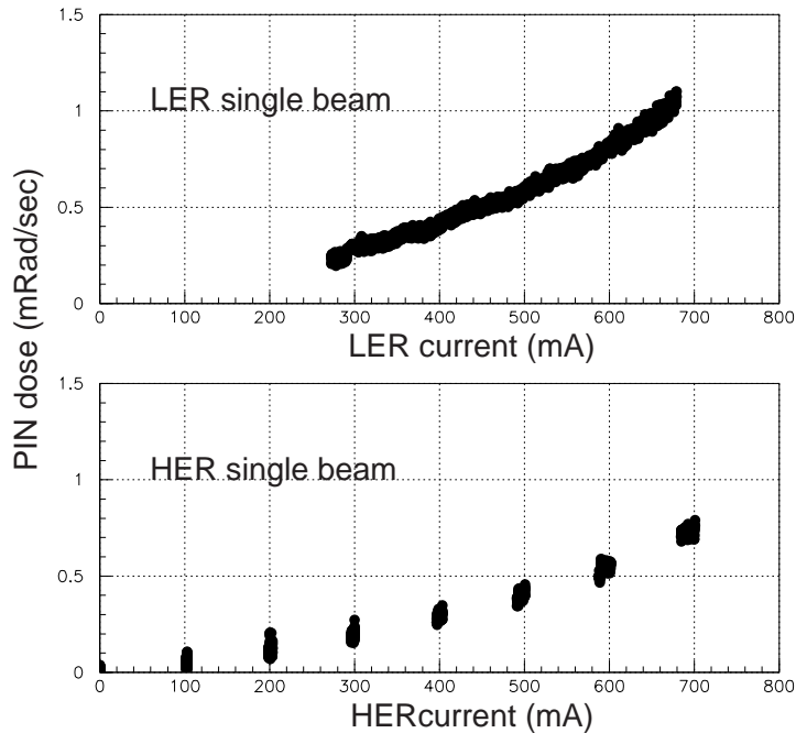
Fig. 30. Background for a single beam. The LER data was taken during a single storage period, while special discrete fills were made for the HER data.
