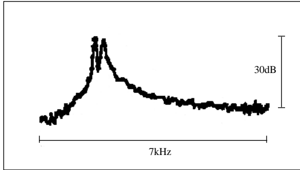
Fig. 14. Beam spectrum observed with a spectrum analyzer. The right and left peaks correspond to the m = -1 and m = 0 betatron modes, respectively.
