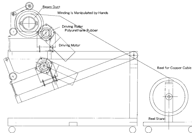
Fig. 44. Coil winding machine for a long solenoid.
