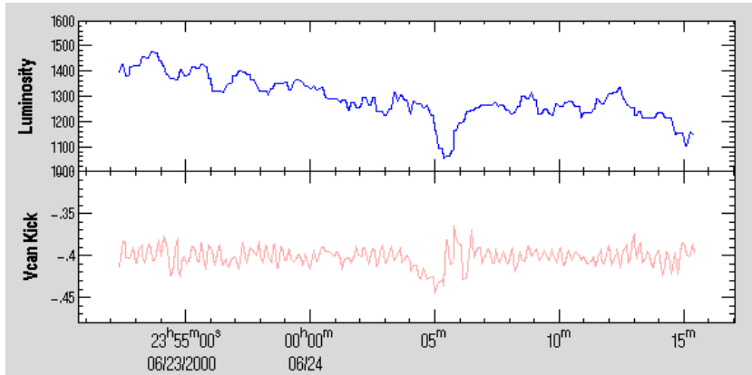
Fig. 26. Luminosity and \Delta x'_{ycan} plotted against time. The feedback for \Delta x'_{ycan} was turned off at 0:03 and luminosity drop followed.
