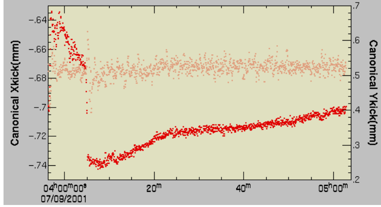
Fig. 25. \Delta x'_{xcan} (dark dots) and \Delta x'_{ycan} (thin dots) for Fill 5931 are shown. The vertical target was kept constant while the horizontal target was changed during the fill. The global trend of \Delta x'_{xcan} is the result of the target change.
