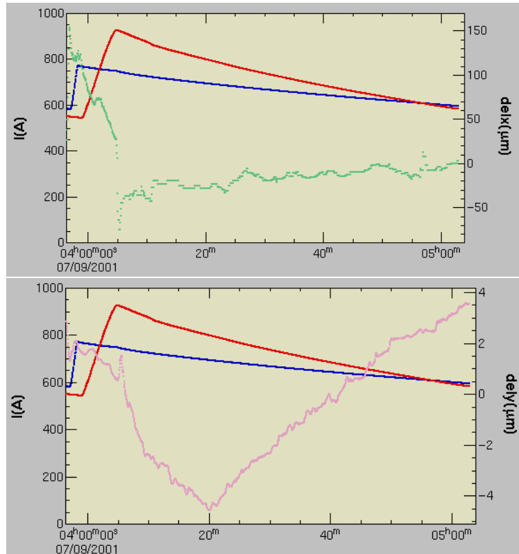
Fig. 24. Horizontal and vertical bump size created by iBump feedback during a typical Fill 5931. The HER and LER currents are also shown in darker lines.
