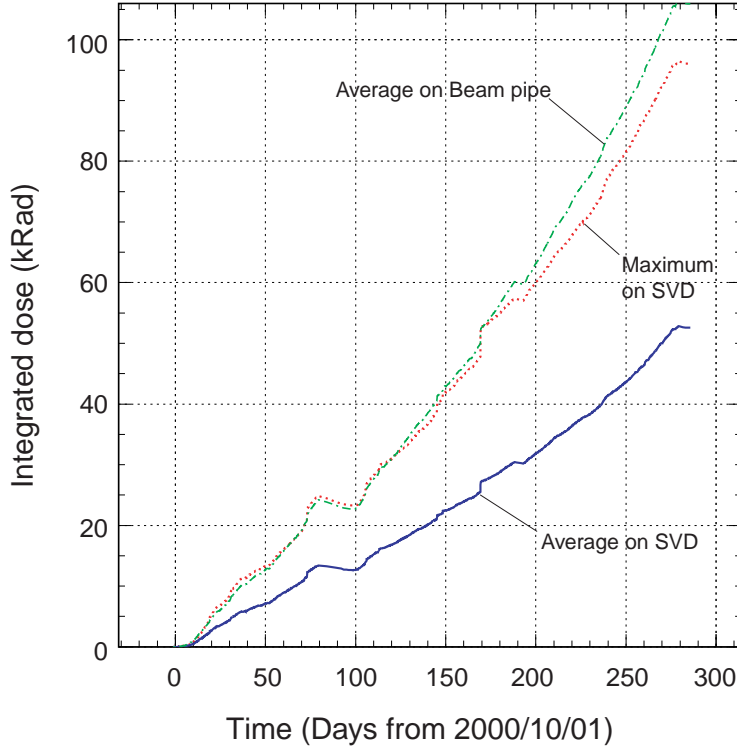
Fig. 29. Accumulated dose measured by RADFETS at the SVD location. The dot-dash curve represents an average dose at the surface of beampipe, The dashed curve and the solid curve show the maximum and the average among the RADFETS at the SVD.
