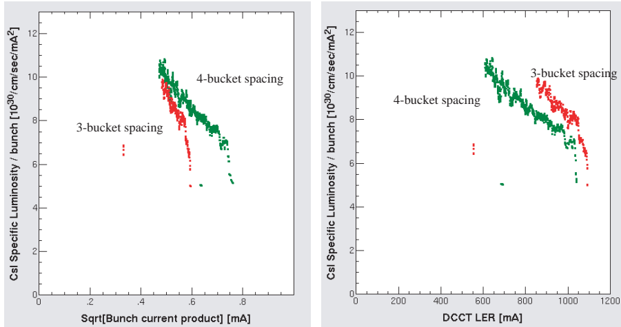
Fig. 17. A specific luminosity as function of a square root of the bunch current product and the LER total beam current. These data were taken on Nov. 9 and 10 in 2001 (after the summer shutdown).
