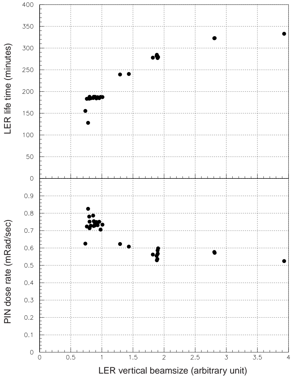
Fig. 33. Background and lifetime as functions of the LER vertical beam The beam size is varied by changing the vertical beam emittance.
