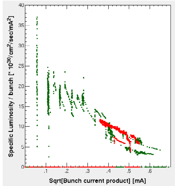
Fig. 18. A current dependence of the specific luminosity with different bunch spacing of 4 bucket(red) and 24 bucket(green). The sepcific luminosity in this figure is somewhat lower than that in Fig. 16 and 17. This is because these data are a bit old and there was some luminosity improvement between after these data had been taken. These two data were taken on the same day (March 10 2001).
