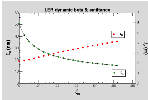
Fig. 20. Calculations of the dynamic beta and dynamic emittance effects with a horizontal tune of 45.51 as function of the (nominal) horizontal beam-beam parameter. The calculation was done by using the SAD code. The solid line shows a beta calculation from an analytical calculation using a simple one-turn transfer matrix.
