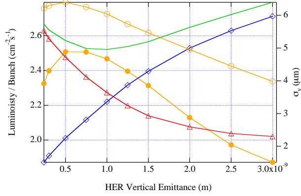
Fig. 28. Luminosity(yellow●), \sigma_y (red △(LER), blue ◇ (HER)) and \Sigma_y (green-) for a crossing angle of 22 mrad and Luminosity(yellow ○) for zero-crossing angle as a function of the HER vertical emittance.
