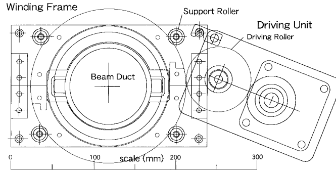
Fig. 45. Coil winding at congested part of the LER beam pipe. after the winding in order to remove the coil.
