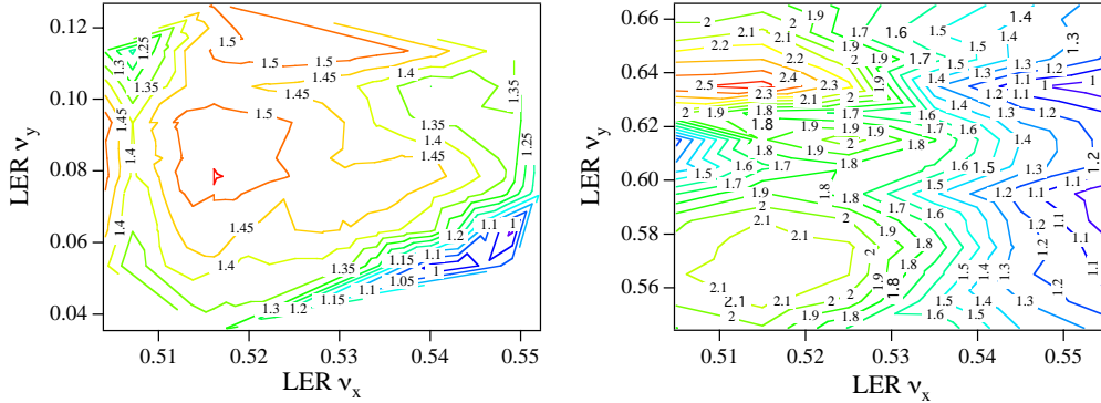
Fig. 21. Results of tune surveys in two different tune regions by using a strong-strong tracking program. The luminosity in the figure is that of a pair of bunches in unit of 10^{30}\text{cm}^{-2}\text{sec}^{-1} . In the tracking, an effect of a finite bunch length was taken into account by slicing the bunches in the longitudinal direction. The number of slices was 5. The tunes of the HER were kept constant; (\nu_x, \nu_y) = (.5136, .6344) in the right figure and (\nu_x, \nu_y) = (.5250, .1350) in the left figure. In the right figure, a luminosity peak near the third integer resonance of the vertical tune is seen. Although we tried this tune region, we could not obtain higher luminosity than the present working point. It turned out that this luminosity peak in the simulation can easily disappear with small errors such as a 0.1 mrad vertical crossing angle.
