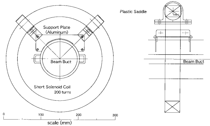
Fig. 43. Frame-less short solenoid coil.
