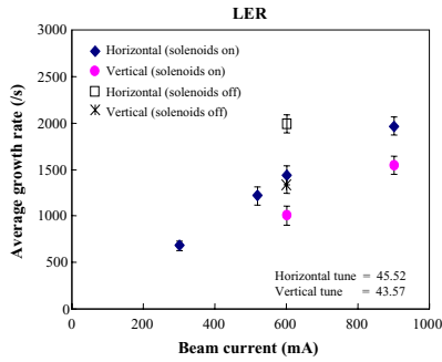
Fig. 10. Average growth rate in the LER.
