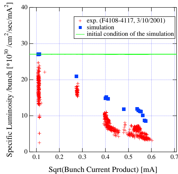
Fig. 19. A comparison of the measured specific luminosity with a 24-bucket bunch spacing to that from the beam-beam simulation using a strong-strong code.
