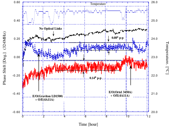
Fig. 3: Long term stability of the E/O-O/E link. A phase stability of \pm 0.04^\circ (324MHz) was obtained for about 6 hours.
