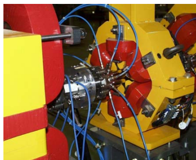
Figure 6: Photograph of the eight-electrodes BPM.
