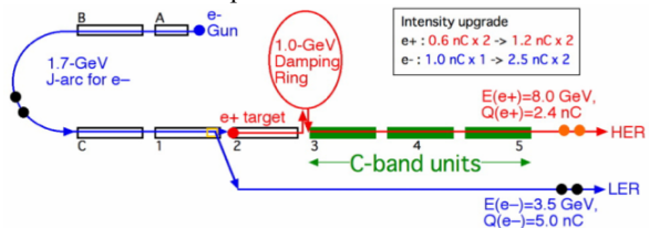
Figure 7: Layout of the linac upgrade for SuperKEKB.
