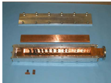
Figure 14: Photograph of the dummy load.
