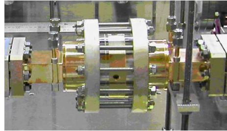
Figure 13: Photograph of the mix-mode window.
