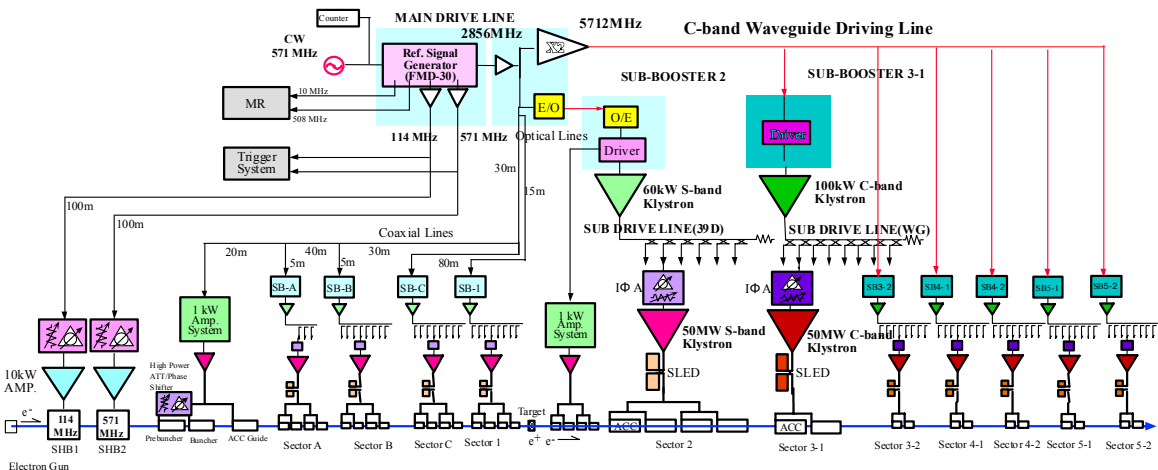
Figure 9: Rf system planned for the linac upgrade.
