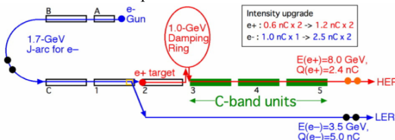
Figure 7: Layout of the linac upgrade for SuperKEKB.
