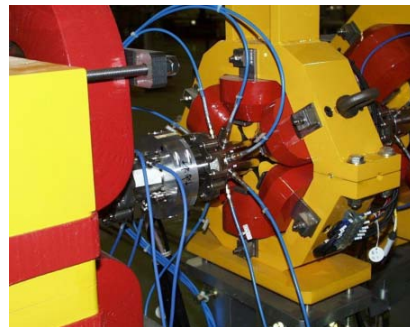
Figure 6: Photograph of the eight-electrodes BPM.
