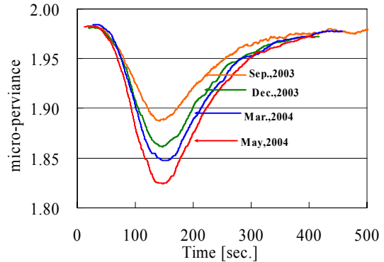
Figure 5: Result of the dip test. This example shows the decrease in emission with time. Such a klystron is replaced prior to a serious emission decrease.
