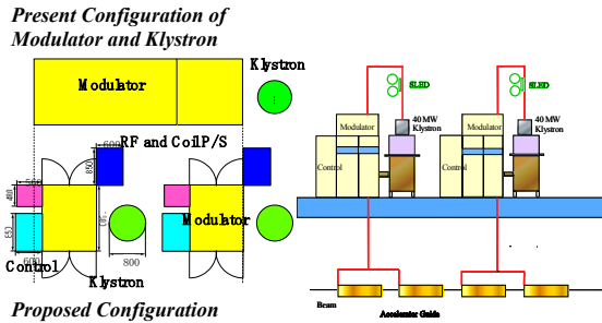
Figure 8: Schematic of the configuration of modulators and klystrons.
