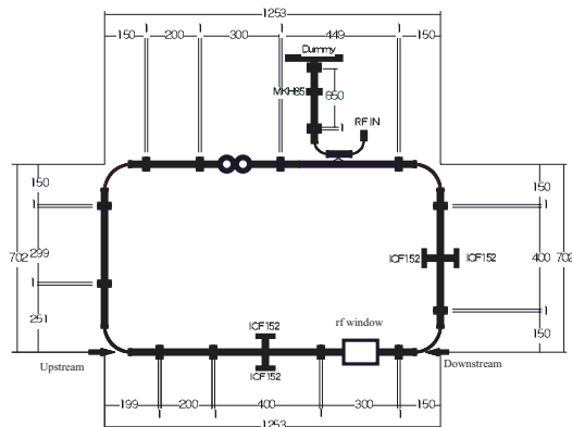
Figure 6: Schematic of the resonant ring.
