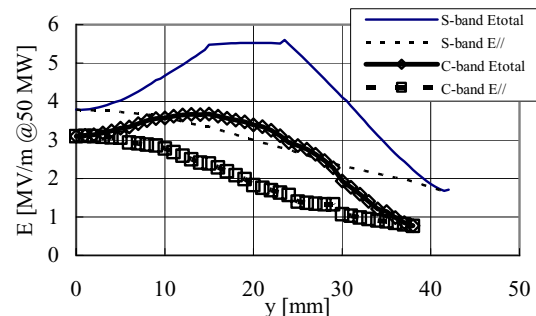
Figure 2: Electric fields on the ceramic disk calculated for C-band and present S-band rf window.
