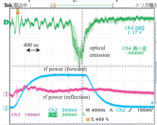
Figure 8: Rf transmission power together with the optical emission.
