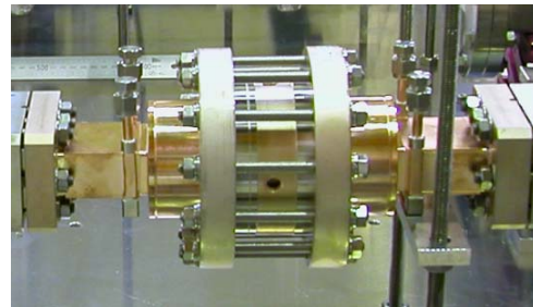
Figure 5: Photograph of the C-band rf window.
