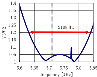
Figure 4: Bandwidth of the C-band rf window.
