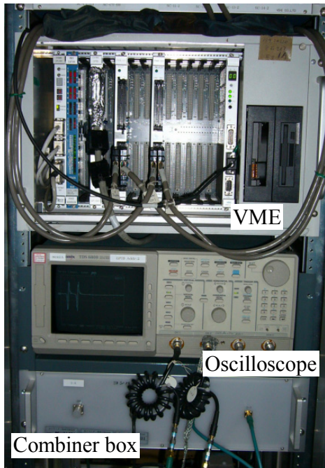
Figure 2: Photograph of previous BPM DAQ system.
