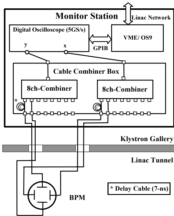
Figure 1: Schematic drawing of previous BPM DAQ system.
