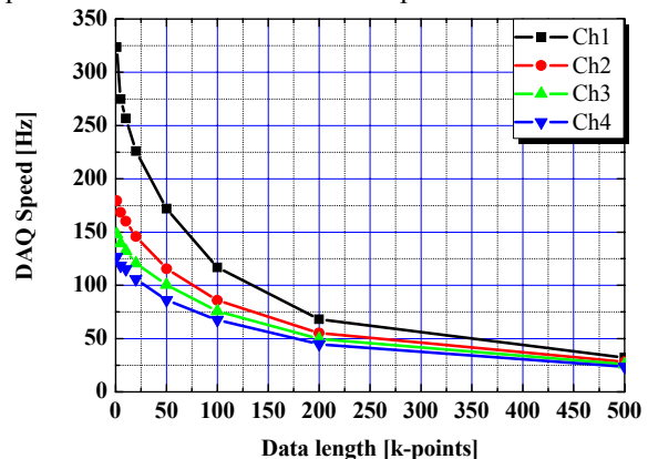
Figure 4: DAQ performance by MSVC++/TekVISA.
