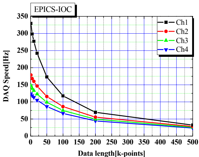
Figure 5: DAQ Performance by EPICS-IOC.
