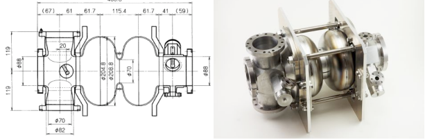
Figure 2: A developed two-cell SC cavity for the injector.
