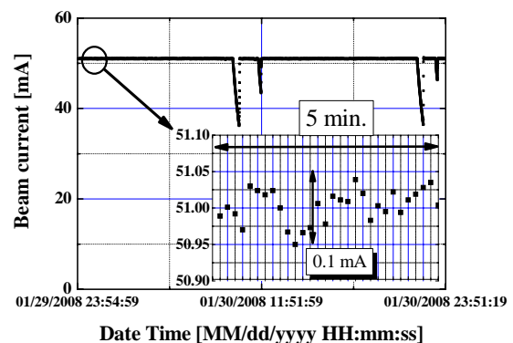
Fig. 4: Stability of stored beam current at PF ring for single-bunch Top-up injection study.
