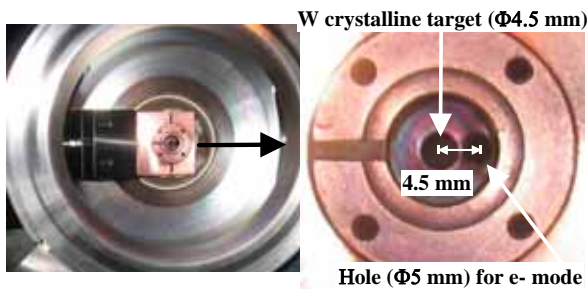
Fig. 2: Photograph of tungsten crystalline positron production target with a hole.
