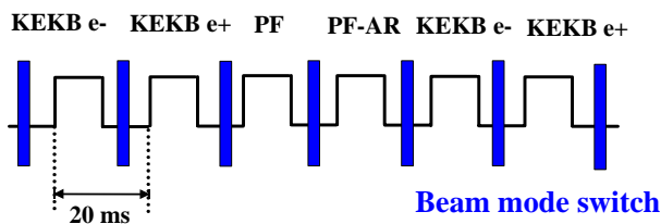
Fig. 1: Schematic drawing of fast beam mode switch.
