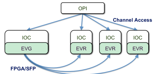
Figure 3: Dual-tier controls with EPICS CA at the top and fast event synchronized control at the bottom.
