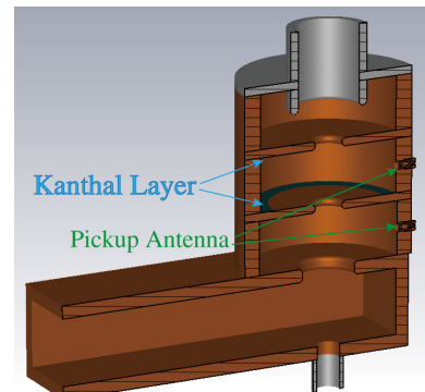
Figure 1: The cross section of the lossy cavity.
