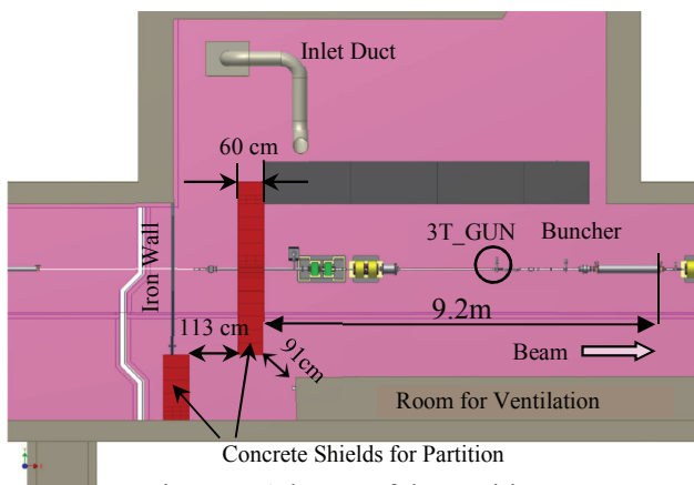
Figure 5: A layout of the partition.
