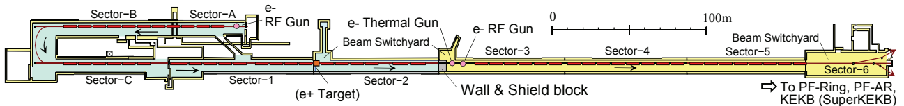
Figure 4: An image of the division of e+/e- Linac. It is separated at the beginning of Sector-3 and ‘down half operation’ is available.
