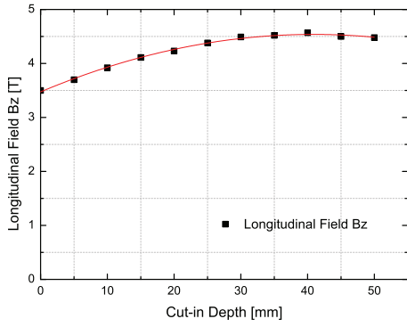
Figure 2: Peak longitudinal field as a function of cut-in cone depth.
