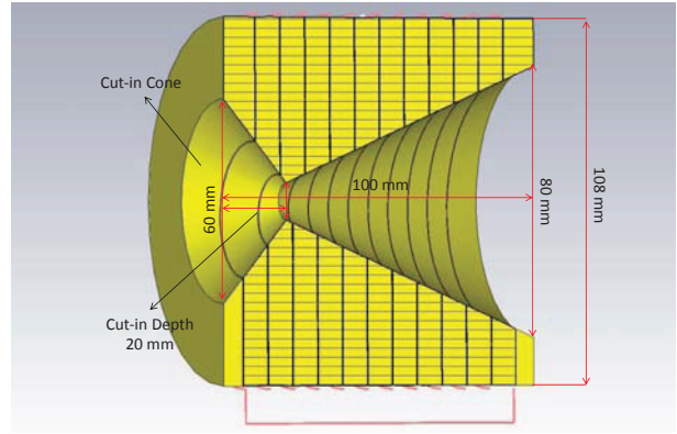
Figure 1: CST Model of the new designed Flux concentrator.
