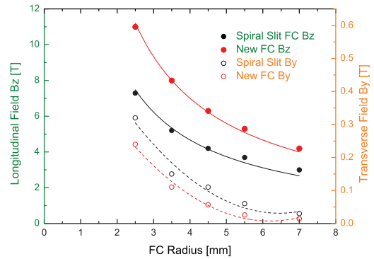
Figure 4: Longitudinal (left y-axis, green color) and transverse (right y-axis, orange color) peak field as a function of FC radius. The longitudinal field and the transverse field are represented by the solid dots and the circles respectively. New FC is shown in red and Spiral slit FC are shown in black.
