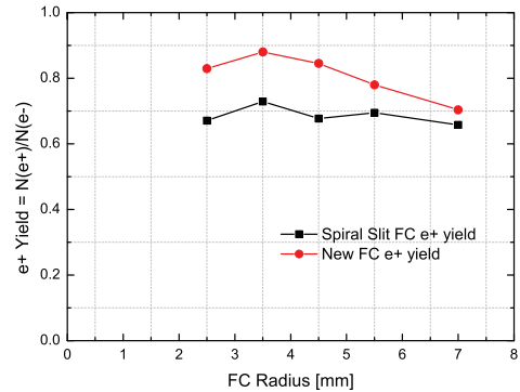
Figure 5: Positron yield as a function of FC radius in the end of capture section. The red and black line represents the new FC and spiral slit FC respectively.
