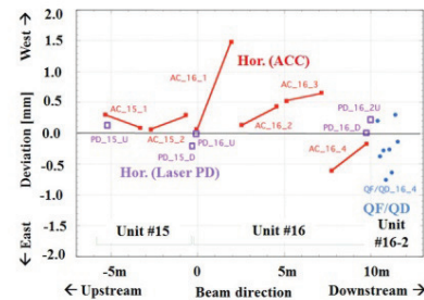
Figure 2: Measured hardware misalignment on a girder.
