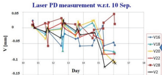
Figure 5: Laser PD measurement along 120m line.
