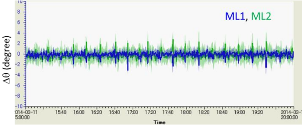
Figure 7: Plot of the detuning angle of the ML cavities.
