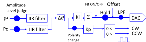
Figure 5: Schematic diagram of tuner control.
