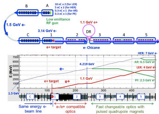
Figure 1: Layout and beam energy patterns of KEK injector linac.
