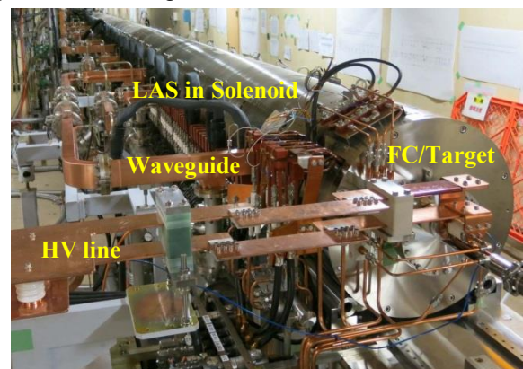
Figure 5: Positron production system.
