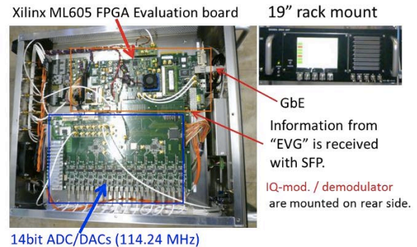
Figure 7: Commonly designed digital RF drive unit and RF monitor.
