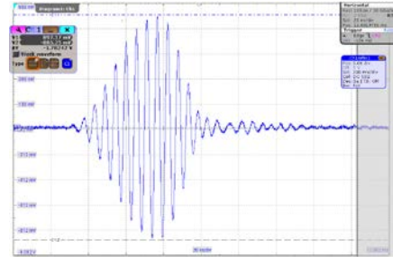
Figure 2: Calibration pulse signal.
