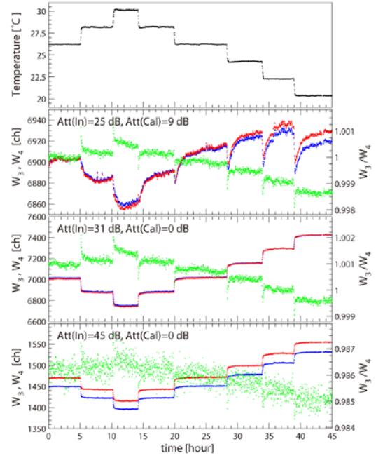
Figure 5: Signal level and gain balance variation.
