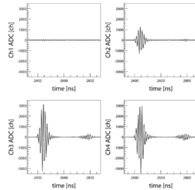
Figure 3: ADC response to the calibration pulse. The pulse was sent to the BPM from Ch1(X+).
