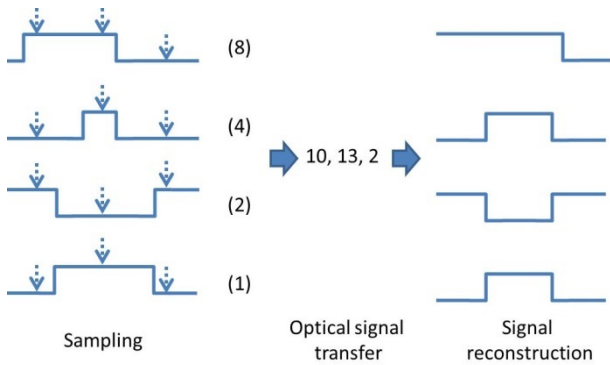
Figure 7: Injection-control signal transfer scheme for SuperKEKB.
