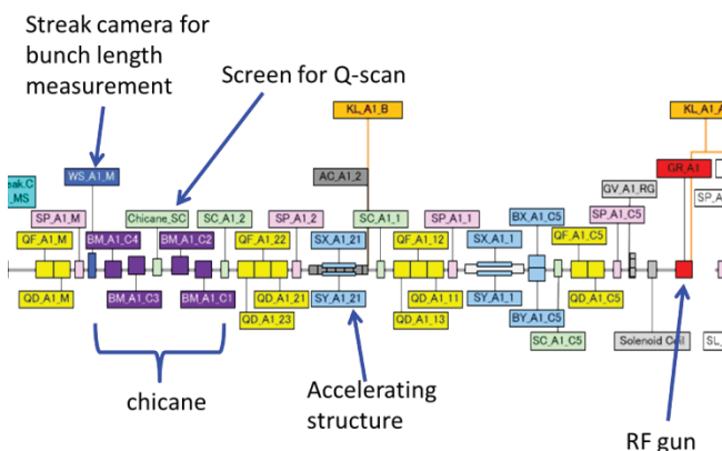
Figure 2: A1 layout.
