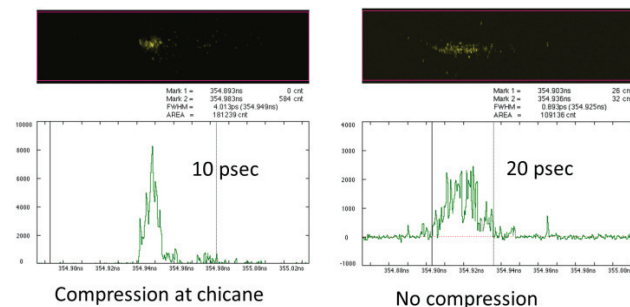
Figure 5: Results of streak camera measurements.
