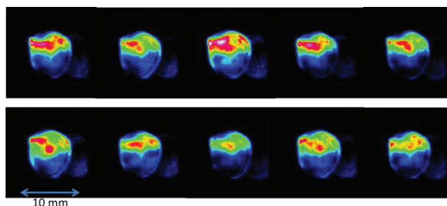
Figure 4: laser profiles of consecutive 10 shot.
