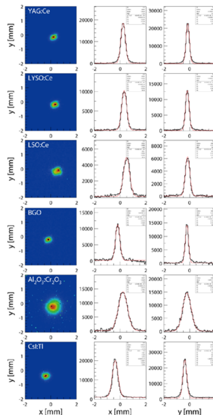
Figure 4: Background corrected beam images and profiles measured with different scintillating screens.
