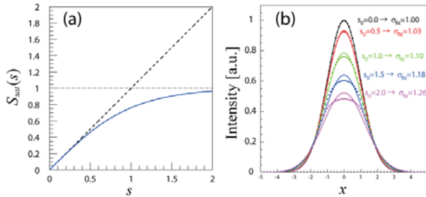
Figure 1: The simple model of the saturation of the luminescence using the equation (1) is shown in the left figure. The right figure shows saturation of the Gaussian distribution. Different levels of the saturation are plotted with different color. The width \sigma_{\text{fit}} obtained from a Gaussian fit (solid line) is represented in the figure.
