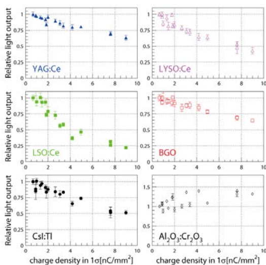
Figure 6: Charge density and relative output of the luminescence. The light output is normalized by the light output of the maximum beamsizes point.
