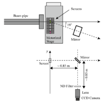
Figure 3: Experimental setup.
