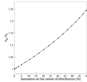
Figure 2: Over estimation of the beam size due to the saturation of the luminescence.
