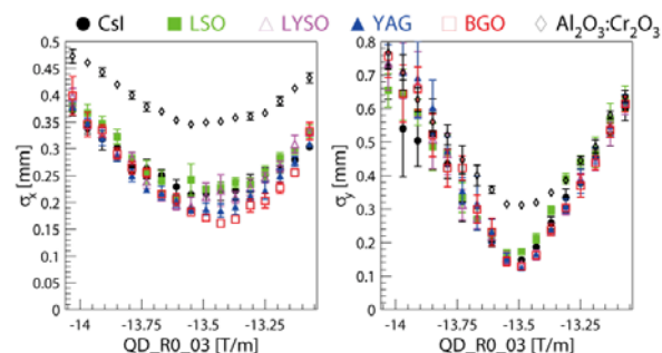
Figure 5: Comparison of electron beam sizes measured with different scintillating screens. The left and right figure show the horizontal and the vertical beam size as a function of the quadrupole strength, respectively. Error bars represent RMS for 10 times measurement of the beam size.
