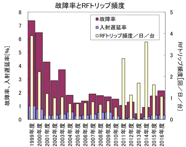
Figure 3: Failure, Injection delay rate and RF trip
