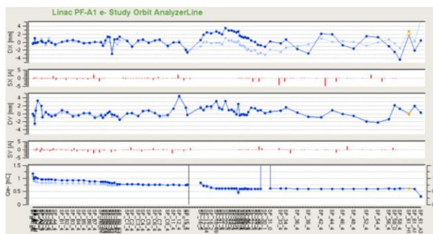
Figure 4: 2 bunches beam transport orbit and charge
