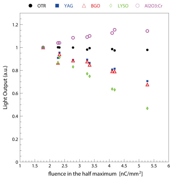
Figure 4: Relative light output, normalized by the most convergent point, and fluence of the beam.
