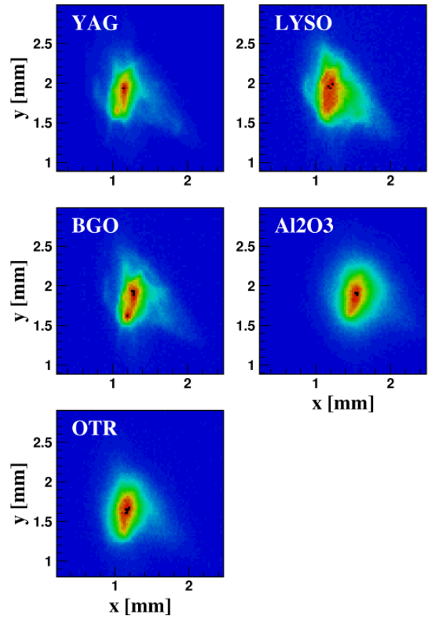
Figure 2: Beam profiles measured by scintillating screens and OTR screen.
