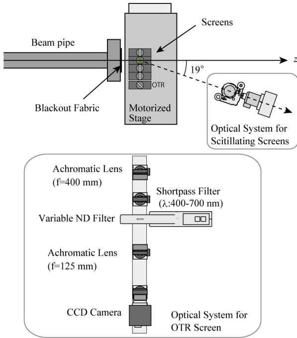
Figure 1: Experimental Setup.
