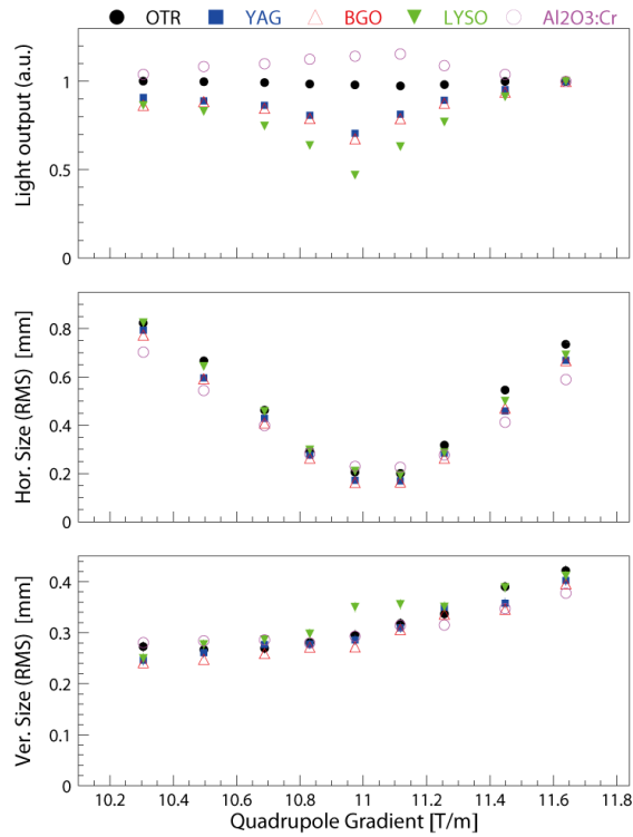
Figure 3: Relative light output and beamsizes as a function of the quadrupole gradient. Plotted data is an average of 10 measurements with the bunch charge of 1.150 \pm 0.005 nC. The light output is normalized by the data at 11.64 T/m.
