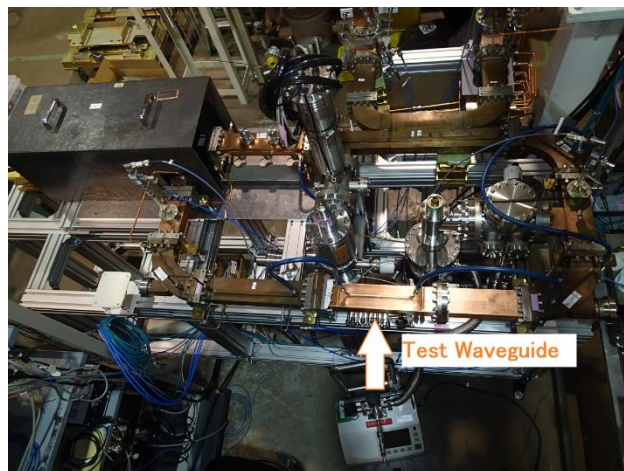
Figure 7: Waveguide under test at the resonant ring.
