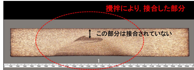
Figure 3: Cut away view of welded test sample.
