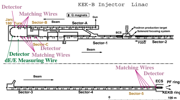
Figure 1: KEKB injector LINAC
