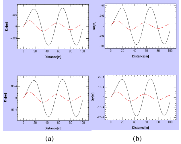
Fig. 2: Simulations for the parametric-excitation nature of the quadrupole wake-field effects in linacs. The betatron oscillations were calculated for the KEKB linac by a simulation based on the two-particle model using the linac parameters given in Table I. The initial conditions are set to x_1 = y_1 = 0 , x_1' = 0.5 mrad, y_1' = 0.01 mrad ( s = 25.4 m), corresponding to the Case II ( Q_s \cong 0 ). (a) W_2 = 0 , and (b) W_2 \neq 0 . The horizontal oscillation increases due to the parametric excitation by about 15% compared to (a), while the vertical oscillation also increases by about 13% through x-y coupling from a large horizontal oscillation. The dashed line shows a simulation without any wake fields.
