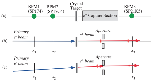
Figure 3: Schematic drawings of the aperture analysis using three BPMs in positron production at the KEBB. (a) Layout of the three BPMs, and schematic orbits of a primary electron and positron beam expected (b) for G = 0 (good orbit) and (c) for G > 0 (bad orbit).
