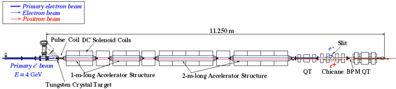
Figure 1: Layout of the positron source at the KEBB injector linac. (QT: quadrupole triplet.)
