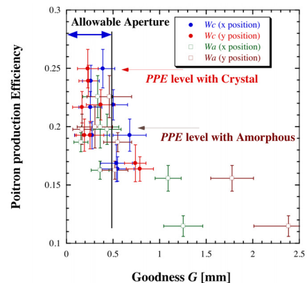
Figure 4: Variations in the PPEs as a function of the goodness G . The data sampled in different time intervals are plotted for both the W_c and W_a targets.
