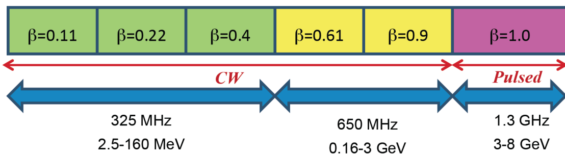
Figure 2: Project X Linac Technology Layout
