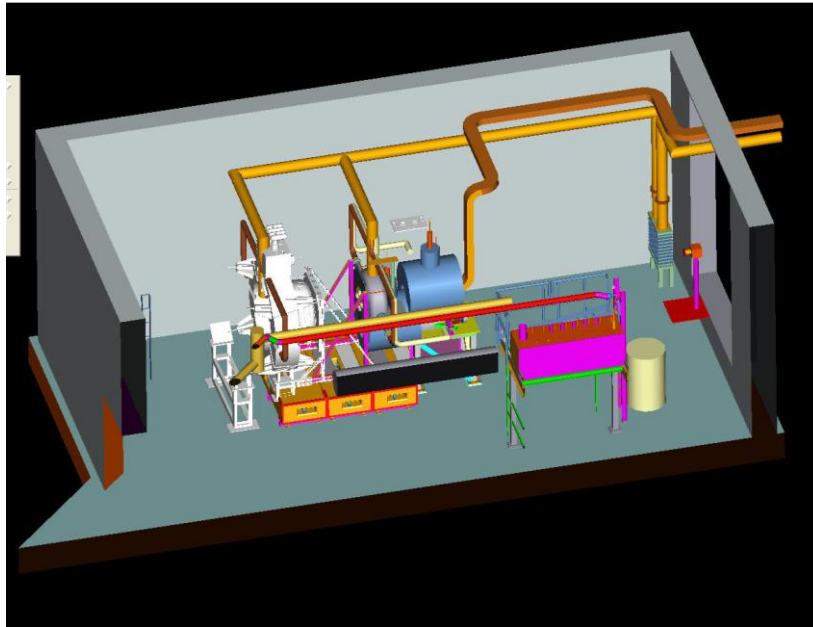
Figure 4: Schematic of MTA hall.
