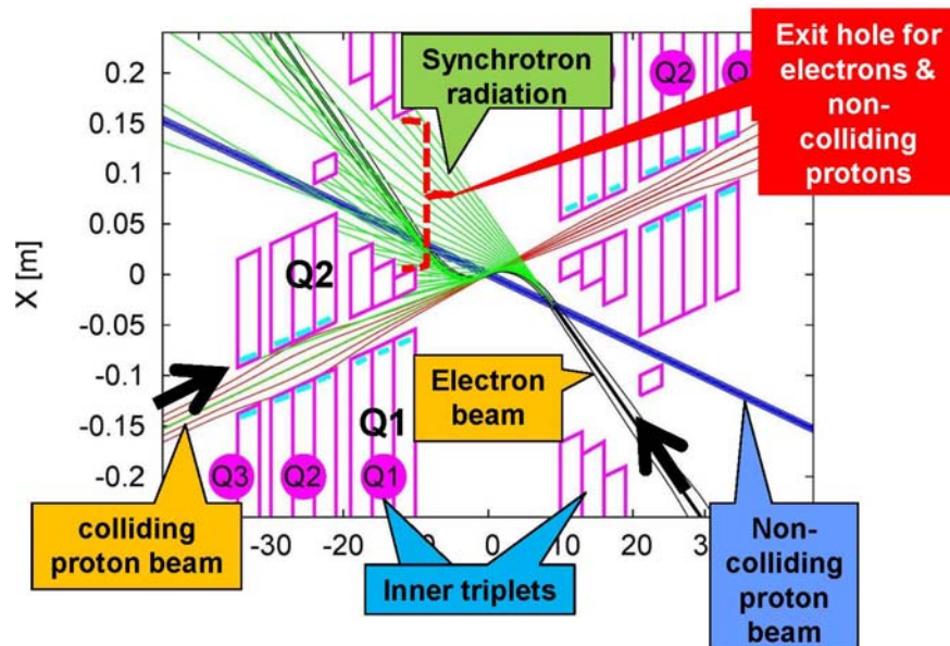
Figure 2: LHeC interaction region with a schematic view of synchrotron radiation [6] (courtesy R. Tomas). Beam trajectories with 5\sigma and 10\sigma envelopes are shown. The parameters of the Q1 and Q2 quadrupole segments correspond to \text{Nb}_3\text{Sn} half-aperture and single-aperture (with holes) quadrupoles.
