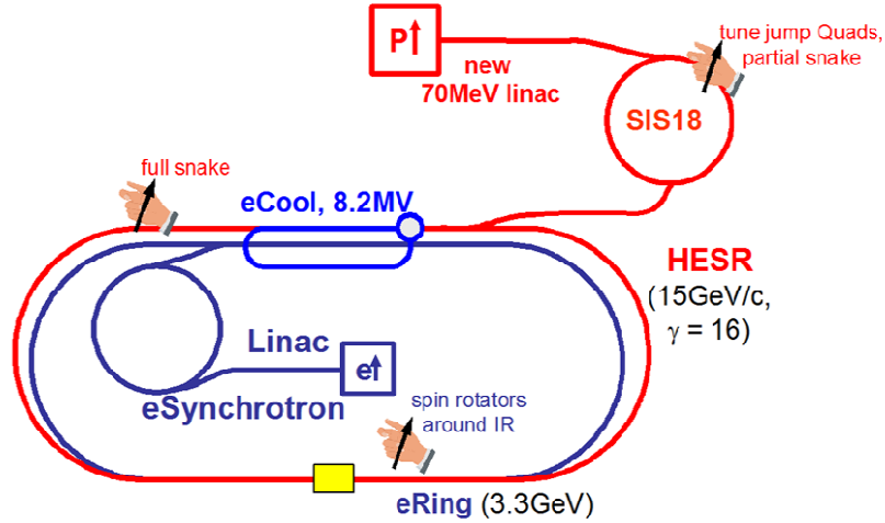
Figure 1: Scheme of ENC at FAIR for electron-proton collisions (not to scale).
