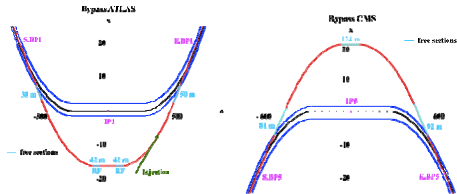
Figure 2: Horizontal bypass in Point 1 and Point 5. The LHC proton ring is shown in black, the electron ring in red and the tunnel walls in blue. Dispersion free sections reserved for the installation of RF, wiggler(s), injection and other equipment are marked in light blue. Beginning and end of the bypass are marked with S.BP and E.BP.
