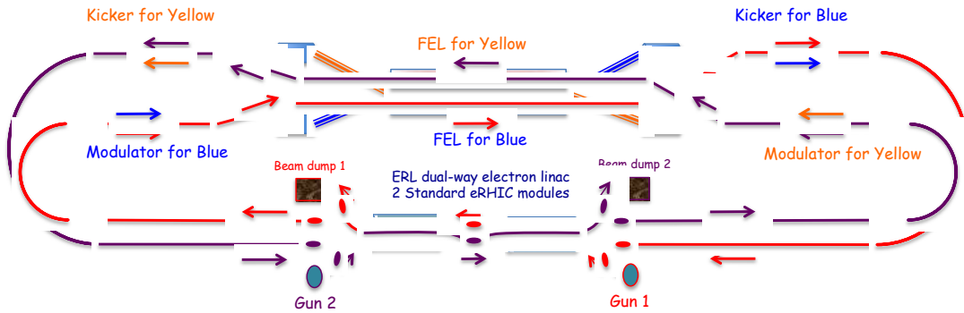
Figure 17: Possible layout of RHIC CeC system's cooling for both the yellow- and blue-beams.
