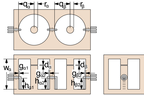
Figure 5: Schematic drawing of BPF structure.
