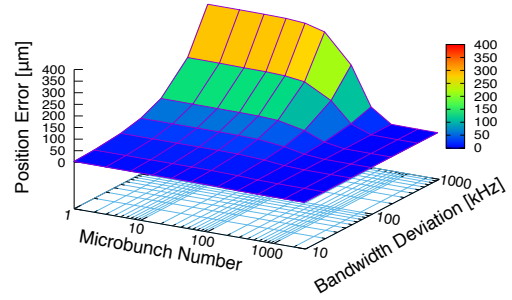
Figure 18: Position error due to bandwidth variation supposing two electrode position measurement and effective aperture radius of 16mm.
