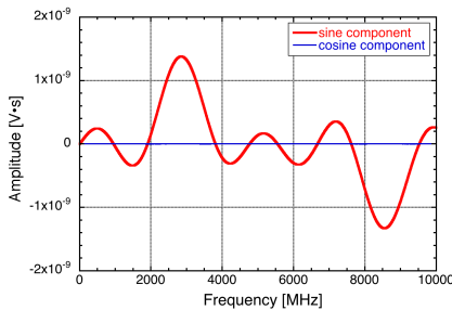
Figure 3: Simulated spectrum given by the Fourier transform of the waveform in Fig. 1.
