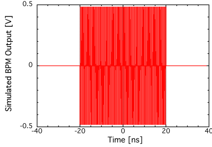
Figure 2: Simulated waveform of the BPM output with -20\text{dB} cable attenuation in the case of 115 microbunches (40ns macropulse width, 1nC/macropulse).
