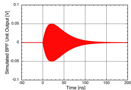
Figure 9: Simulated waveform given by the inverse Fourier transform of the spectrum in Fig. 7 (1ns macropulse width, 1nC/macropulse).
