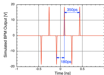
Figure 1: Simulated waveform of the BPM output with -20\text{dB} cable attenuation in the case of three microbunches (1ns macropulse width, 1nC/macropulse).
