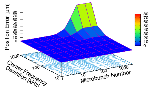
Figure 15: Position error due to center frequency variation supposing two electrode position measurement and effective aperture radius of 16\text{mm} .
