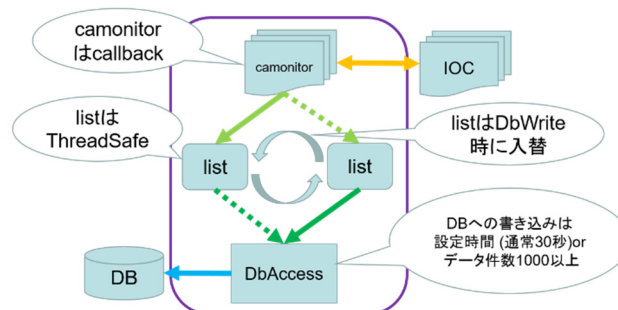
Figure 3: Writer thread block diagram.
