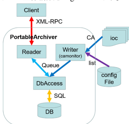
Figure 1: Portable Archiver block diagram.
