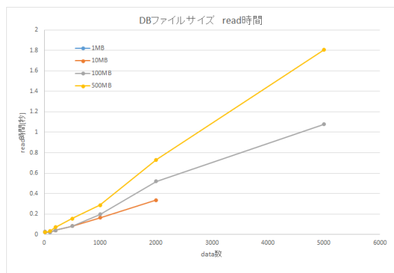
Figure 5: Read performance vs DB file size.
