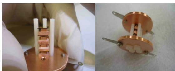
Figure 5: Cascade stuck using the SiC-DSRD bare chips.
