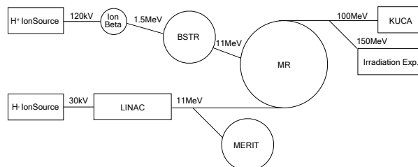
Figure 1: Layout of the KURNS FFA Complex.
