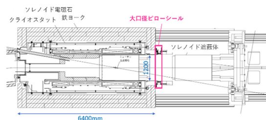
Figure 2: Drawing of a large-diameter pillow-seal and a solenoid magnet with a radiation shielding unit.
