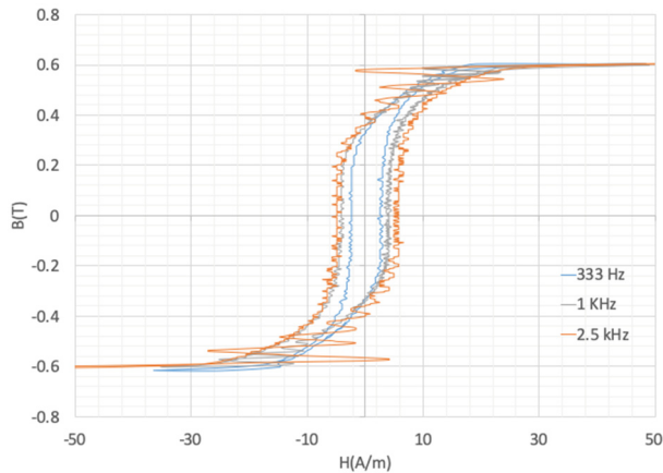
Figure 3: RT core hysteresis curve at different frequencies.
