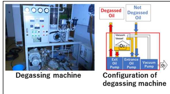
Figure 8: Degassing.
