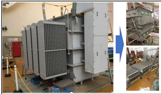
Figure 6: Removing radiators.
