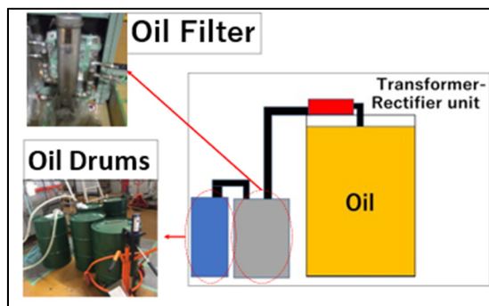
Figure 7: Filling oil.
