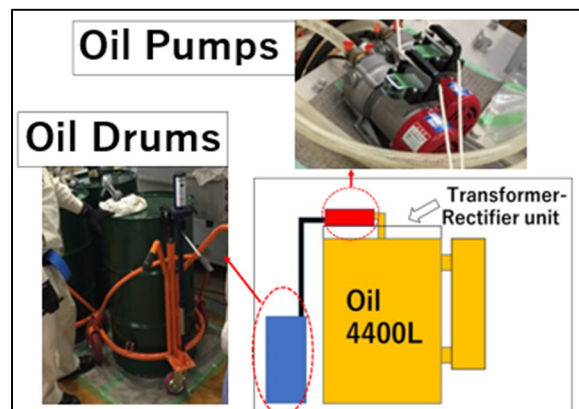
Figure 5: Removing oil.
