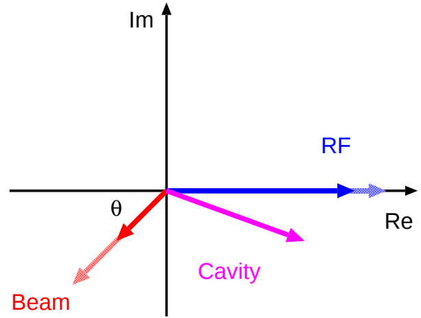
Figure 3: Phase diagram of RF term (blue) and Beam term (red) with phase \theta . The solid and hatched arrows show the instantaneous and the asymptotic values.
