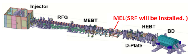
Figure 2: Configuration of long pulse beam commissioning [2].
