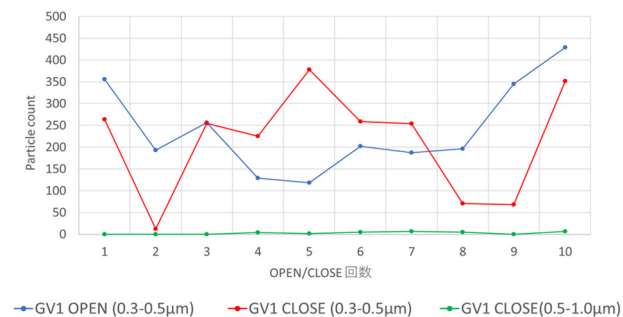
Figure 8: Result of particle measurement in MEBT side vacuum chamber.
