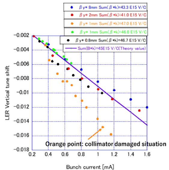
Figure 3: LER vertical tune shift versus bunch current.
