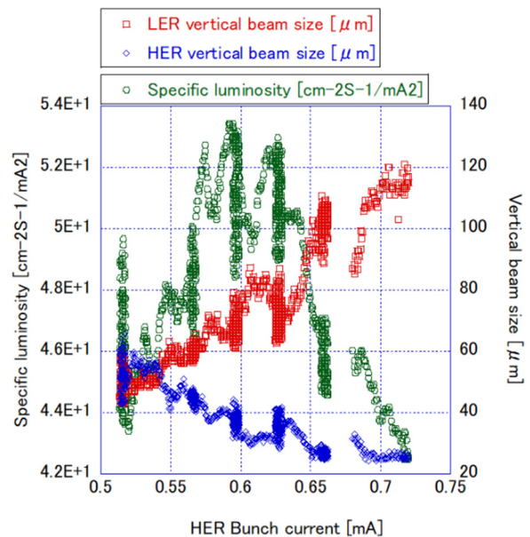
Figure 13: The result of high bunch study during collision situation.
