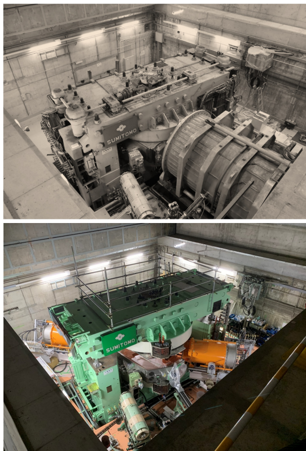
Figure 1: Top views of AVF Cyclotron at RCNP. Upper figure shows the cyclotron before upgrade, and bottom shows the one after upgrade.
