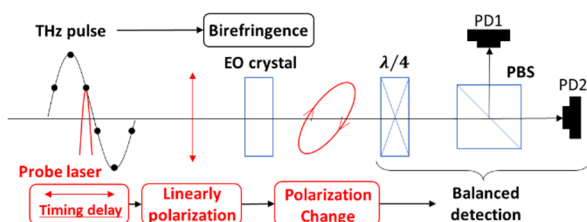
Figure 5: Principle of EO sampling.
