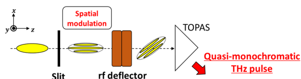
Figure 4: Quasi-monochromatic THz pulse generation.
