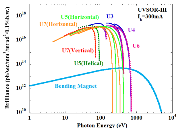
Figure 3: Synchrotron radiation spectra of UVSOR-III.
