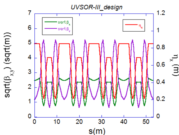
Figure 2: Betatron and dispersion functions of UVSOR-III.
