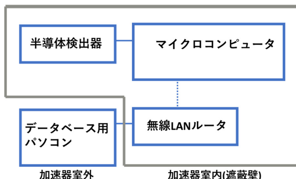
Figure 1: Schematic diagram of the measurement system.
