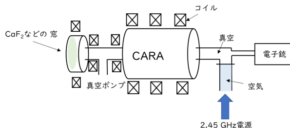
Figure 3: Schematic diagram of test bench CARA.
