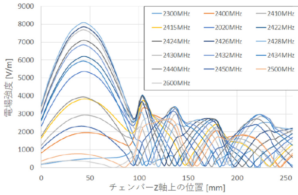
Figure 6: Electric field each frequency (2300~2600 MHz) simulated by HFSS.
