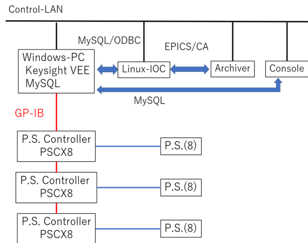
Figure 2: Schematic drawing of the current control system for magnet power supplies with GP-IB and customized controller (PSCX8).
