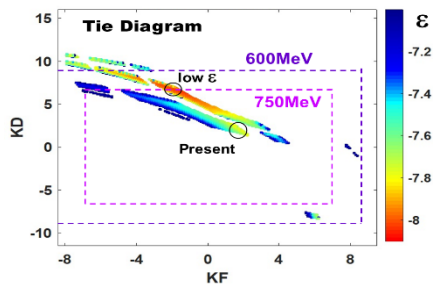
Figure 2: Tie diagram of UVSOR-III magnetic lattice. KF and KD are quadrupole strengths, B'/B\rho . The hardware limitations of the quadrupole magnets are indicated by dashed lines for two operating energy, 750 MeV and 600 MeV. The emittance is indicated by the colour in the logarithmic scale. The operating areas of the present optics and the low emittance optics are indicated by black circles.
