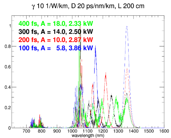
Figure 4: Input pulse duration dependence.
