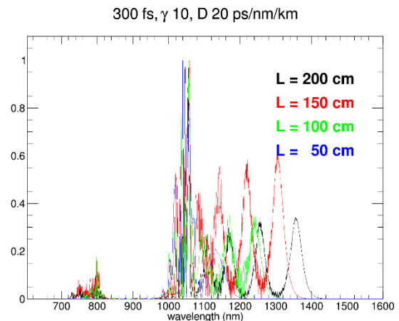
Figure 5: Fiber length dependence.
