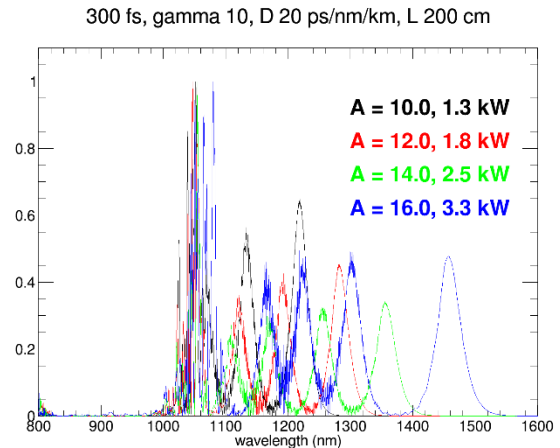
Figure 3: Input power dependence of the output of HN-PCF-1040.
