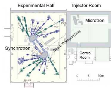
Figure 1: HiSOR accelerators and SR experimental hall.
