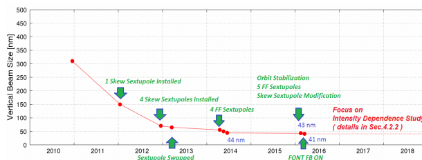
Figure 5: History of the smallest beam size achieved at the ATF2 focal point.
