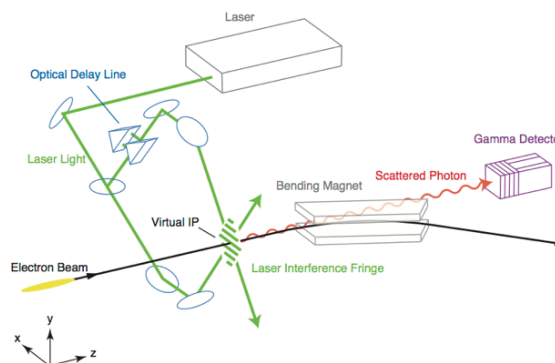
Figure 3: Schematic configuration of the nanometer beam size monitor at ATF2.
