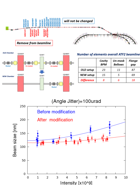
Figure 6: Beam size measured at the focal point of ATF2, before and after the reduction of wakefield sources.
