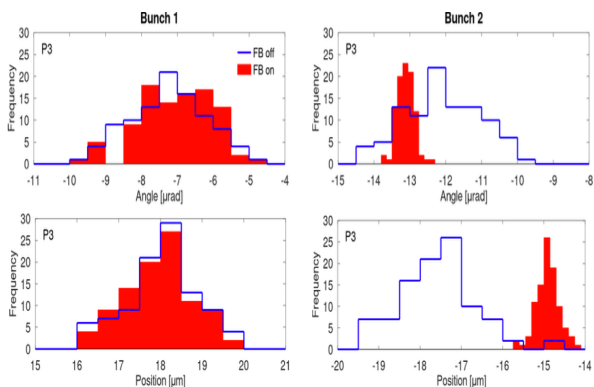
Figure 9: Intra-train feedback at ATF2. Bunch 1 shows the input of feedback and bunch 2 shows the result. Upper plots are for angle of bunch trajectory and lower plots are for bunch position.
