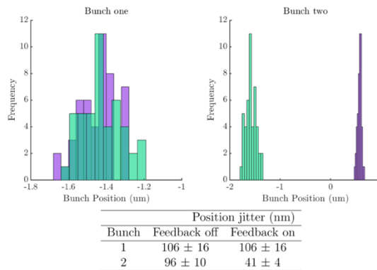
Figure 10: Beam position at IP BPM w/o FONT.
