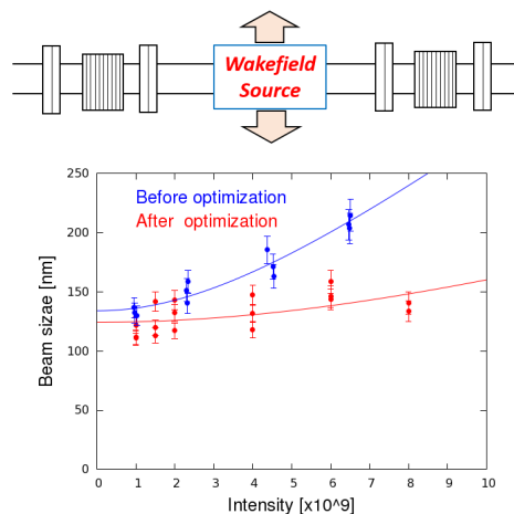
Figure 7: Reduction of the wakefield effect on a small beam at ATF2, by optimizing the position of an additional wakefield source.
