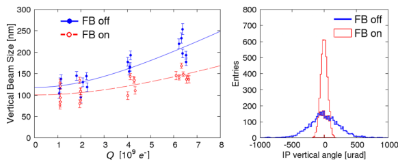
Figure 11: Improvement of beam intensity dependence by EXT-FONT feedback.
