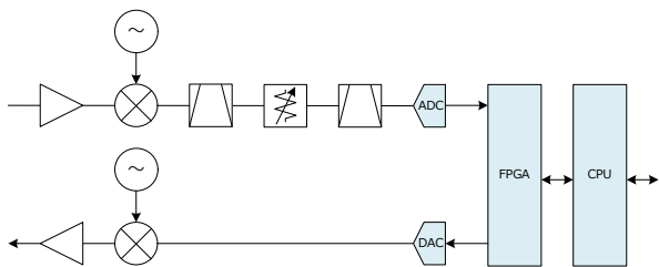
Figure 1: Block diagram of current high-frequency signal processing.
