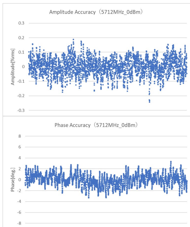
Figure 11: Amplitude and phase accuracy when sampling at 5712 MHz and narrowing to BW ±1 MHz.
