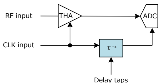
Figure 5: Block diagram of clock delay adjustment circuit.
