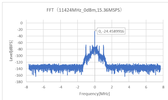
Figure 9: Spectrum when sampling at 11424 MHz and narrowing to BW ±1 MHz.
