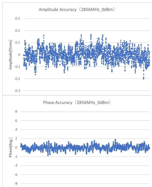
Figure 12: Amplitude and phase accuracy when sampling at 2856 MHz and narrowing to BW ±1 MHz.
