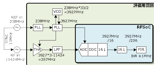
Figure 6: Block diagram of X-band high frequency signal monitor evaluation.
