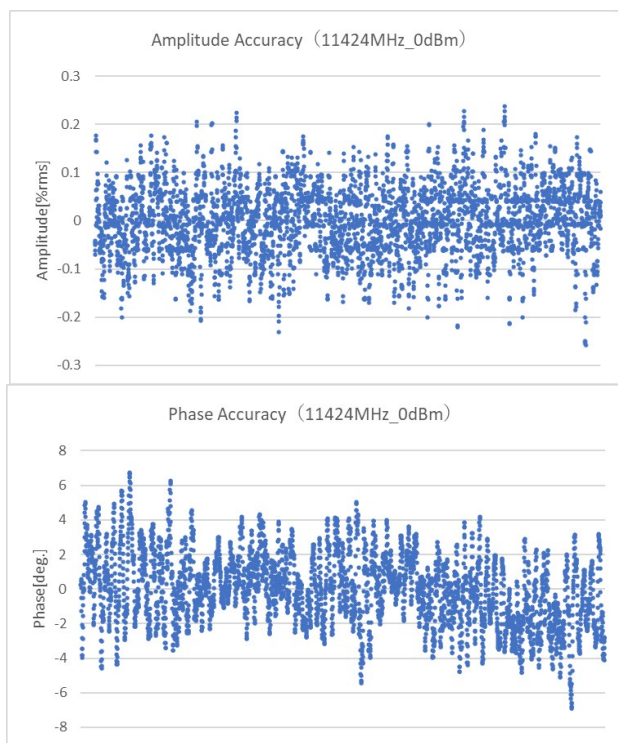
Figure 10: Amplitude and phase accuracy when sampling at 11424 MHz and narrowing to BW ±1 MHz.
