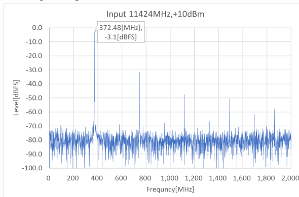
Figure 8: FFT spectrum during X-Band signal input.
