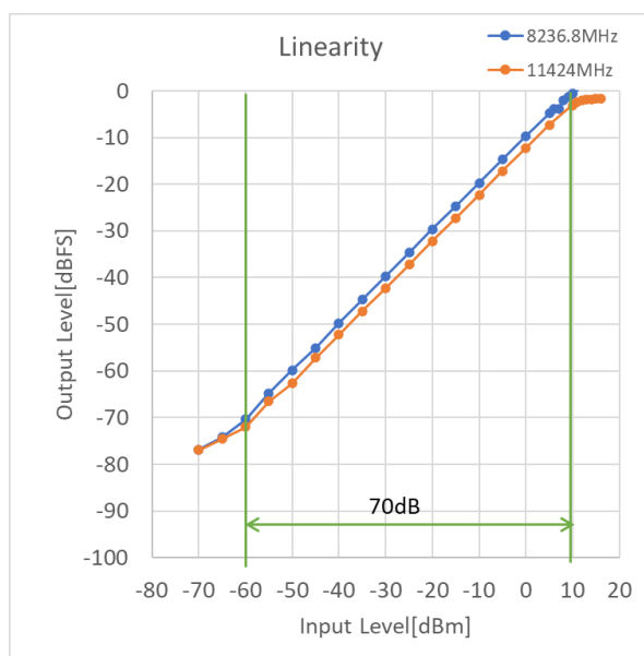
Figure 7: Linearity evaluation results of ADC with X-Band signal input.
