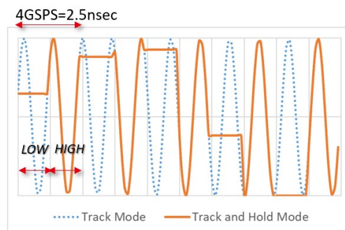
Figure 4: Overview of track and hold mode in THA.
