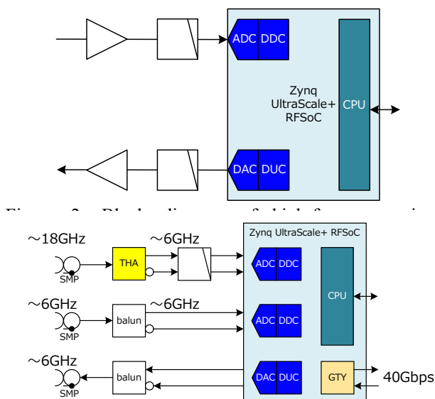
Figure 3: Block diagram of X-band RF signal monitor circuit.
