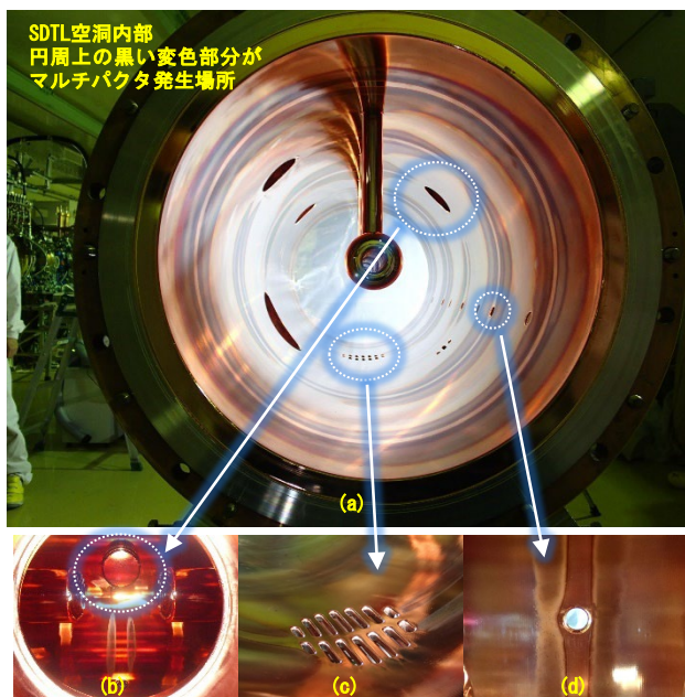
Figure 1: Inside photo of the SDTL05B cavity.
