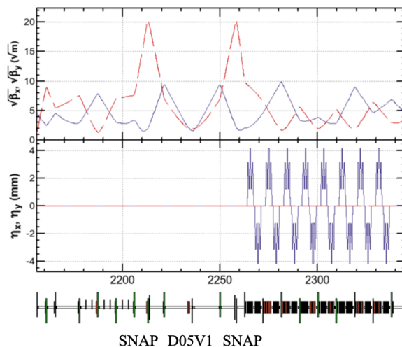
Figure 3: Optics of nonlinear collimator section.
