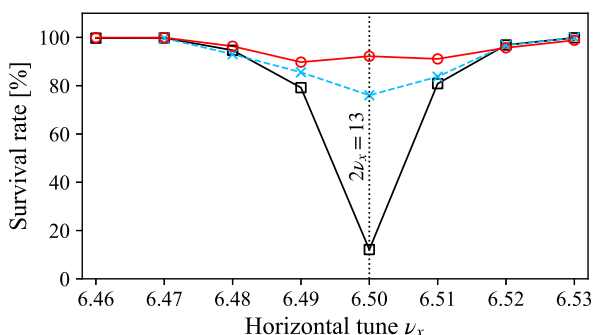
Figure 9: Horizontal tune dependence of the particle survival rate after 4 ms from the injection with the vertical tune was set at 6.36.
