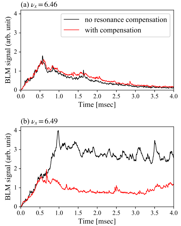
Figure 11: BLM signals over the first 4 ms measured in the collimator section with (red) and without (black) the addition of the QDTs at the operating point of (a) (\nu_x, \nu_y) = (6.46, 6.36) and (b) (6.49, 6.36) .
