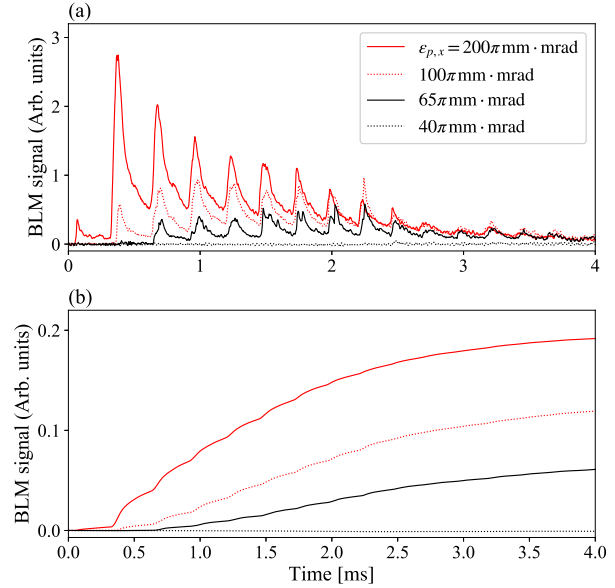
Figure 4: (a) BLM signals over the first 4ms measured in the collimator section with 4 different injection painting areas in the horizontal plane and (b) integrations of them.
